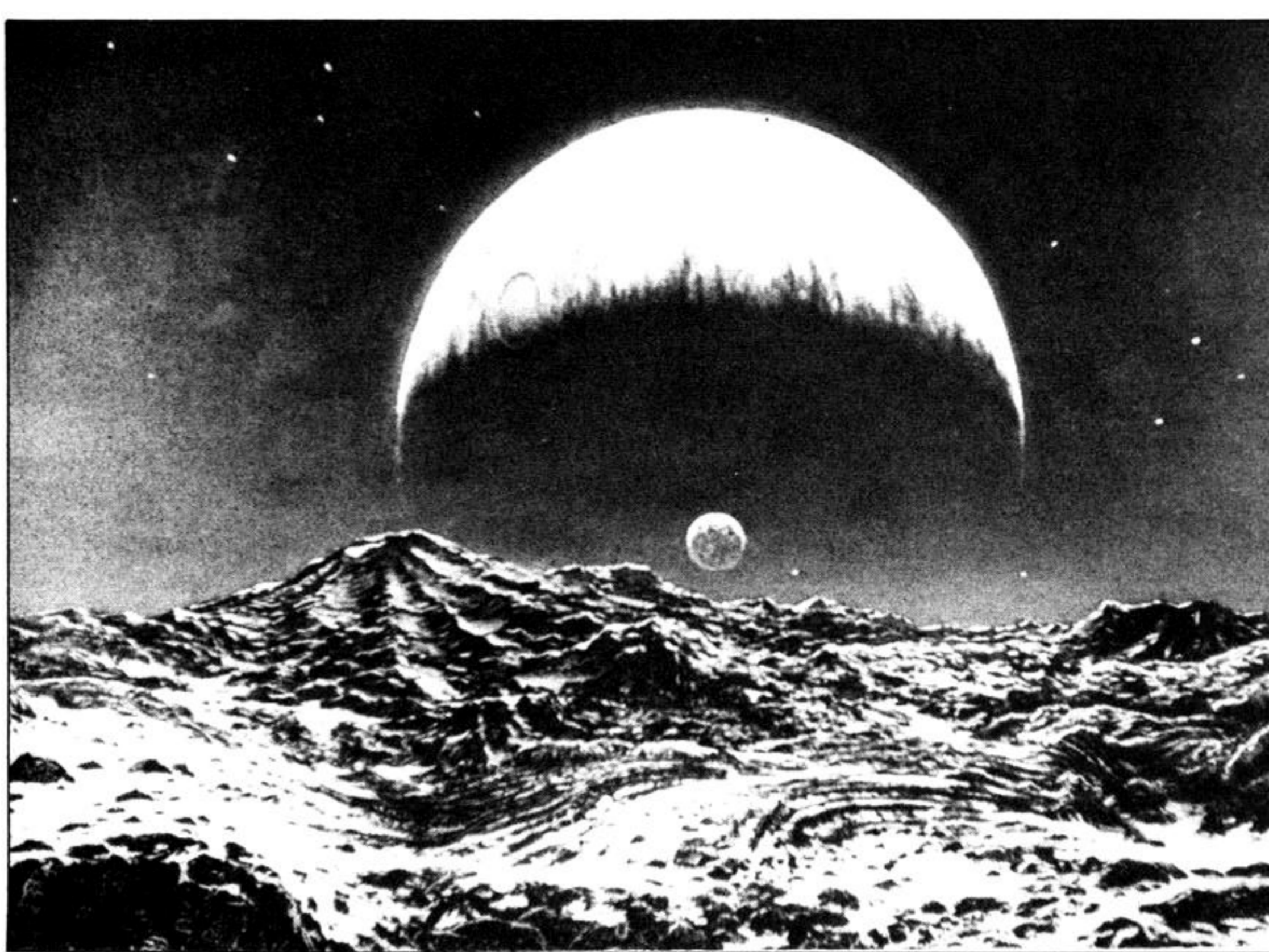
Above: Jupiter is the largest of all the planets and, according to some scientists, almost became a star itself. Here it rides majestically in the sky of Europa, one of its large moons, as a closer satellite, Io, rises above the rocky horizon.
